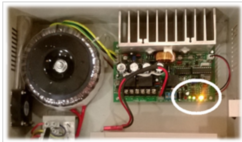
LED on PCB inside NAYAtel 70W UPS metallic body (with lock)
